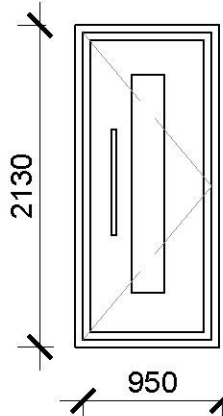
PROPOSED FRONT DOOR
