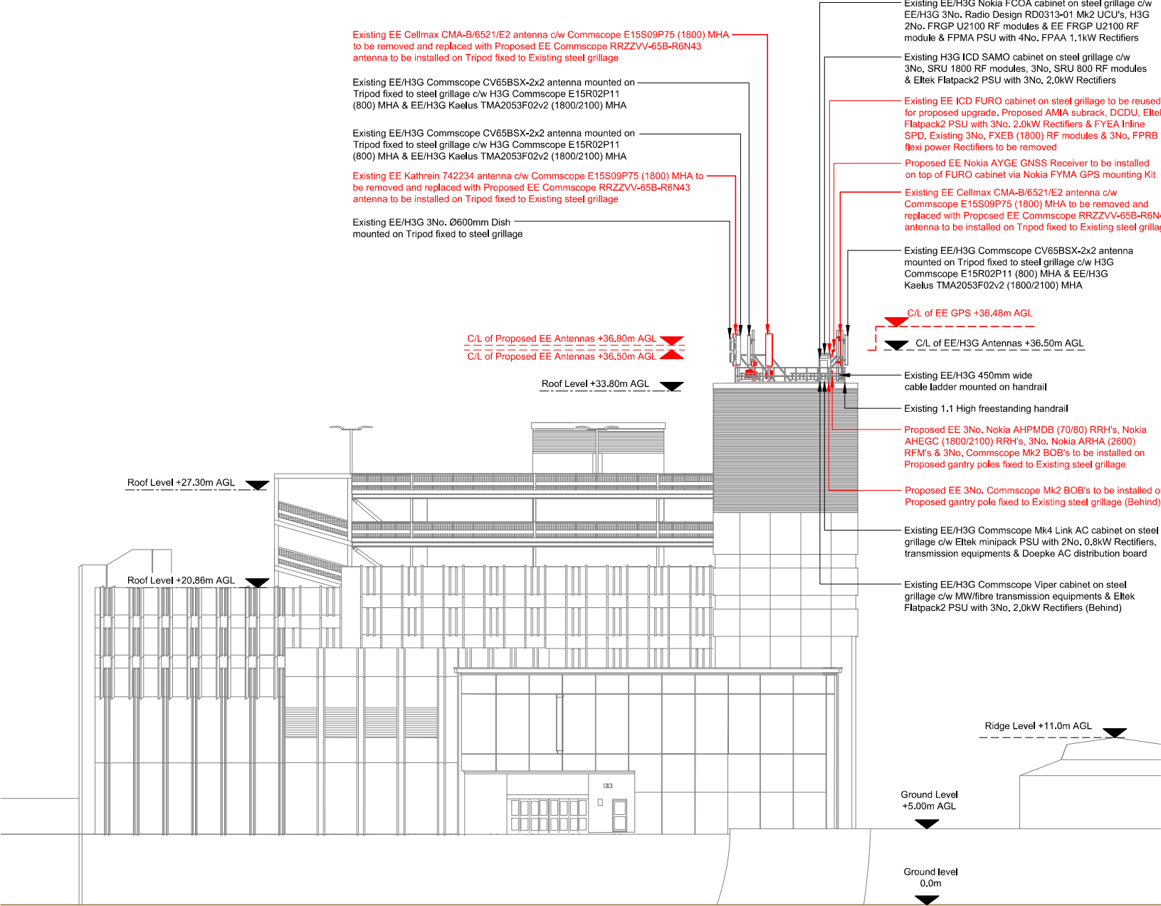
PROPOSED SITE ELEVATION A 0 1:250 5m 10
