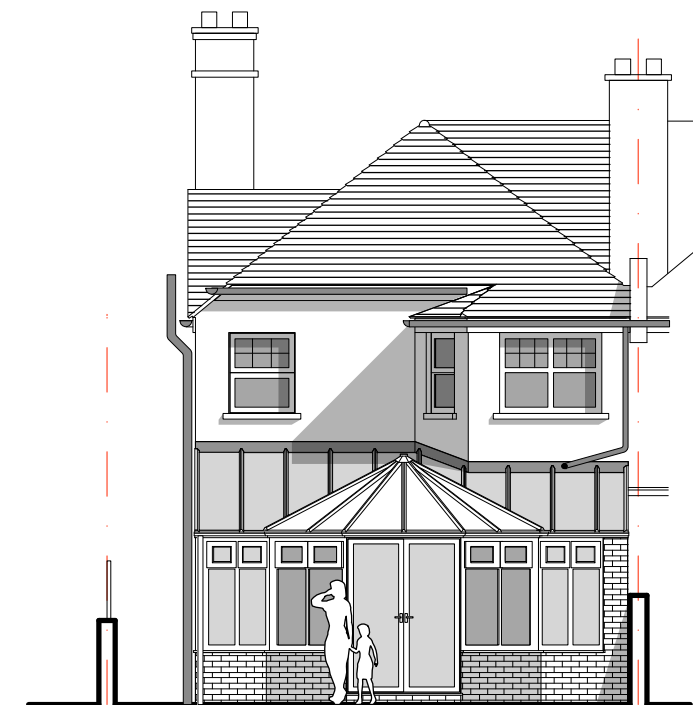
02 Rear Elevation As existing
