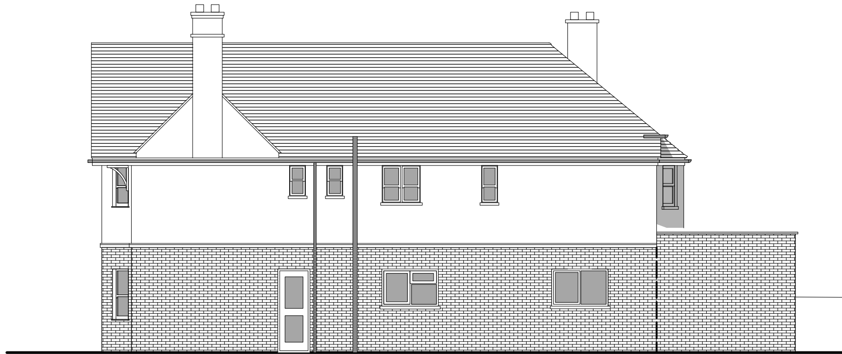
01 Side Elevation As proposed
