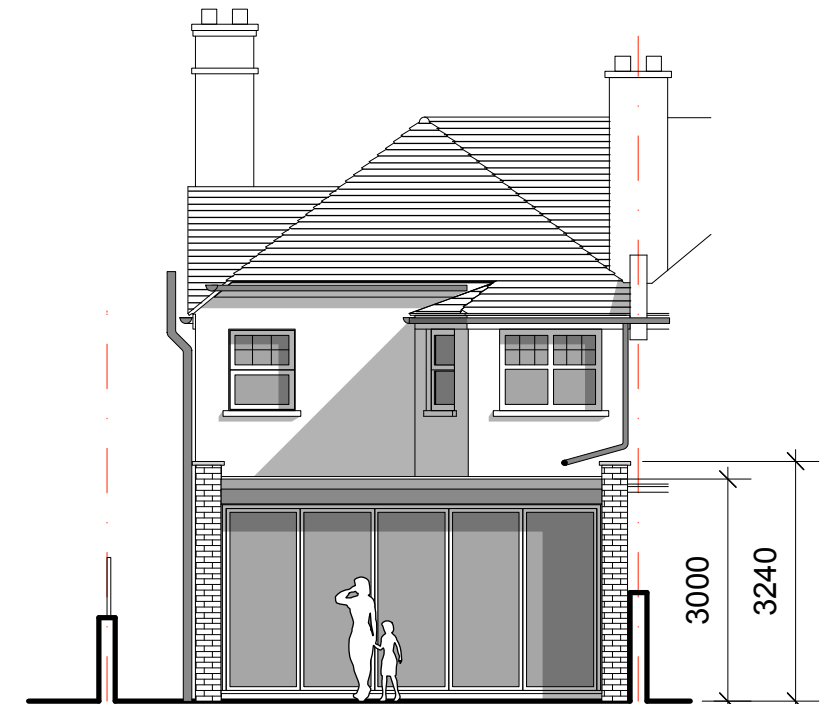
02 Rear Elevation As proposed
