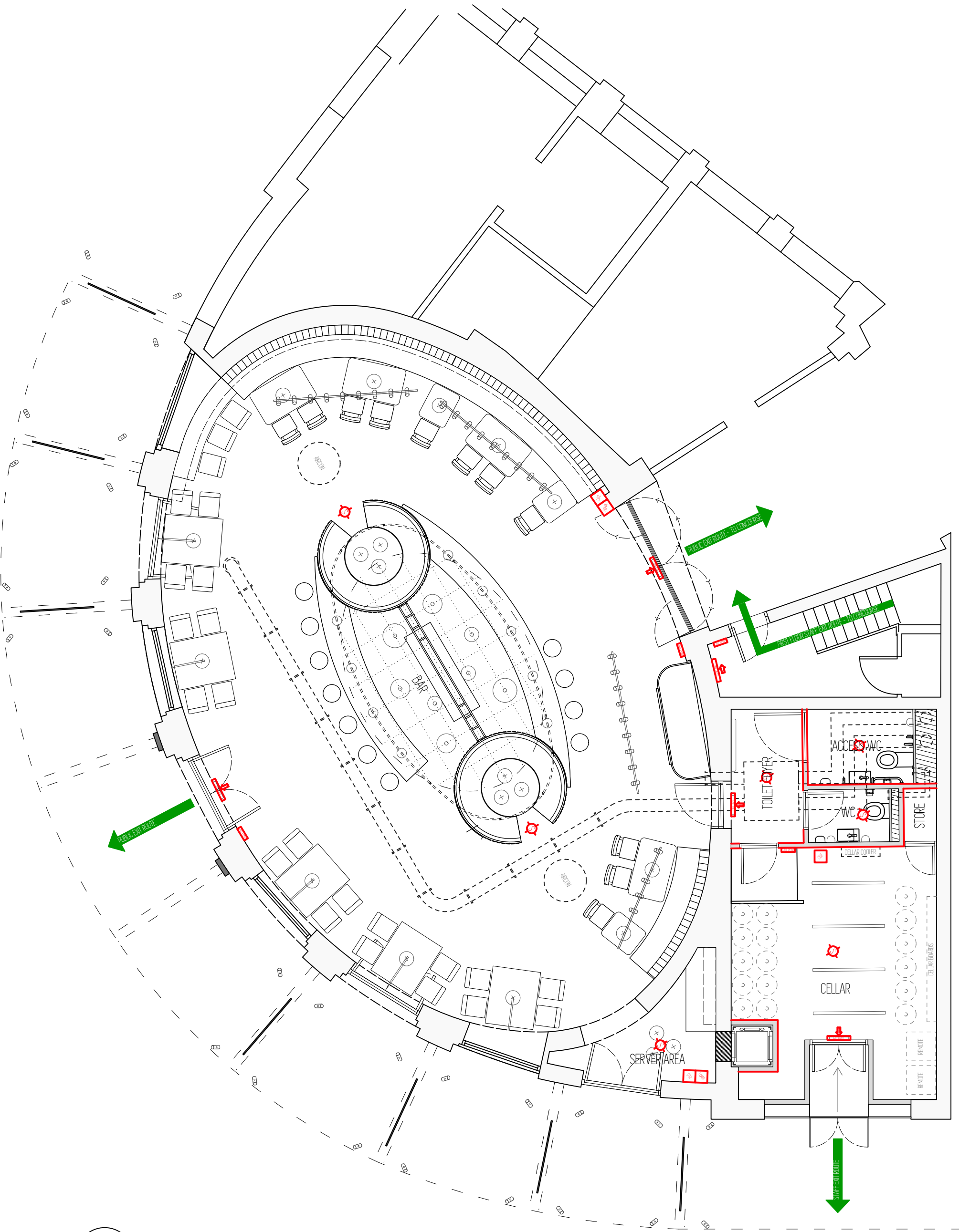
009/1 FIRE PROTECTION GROUND FLOOR Scale: 1:75
